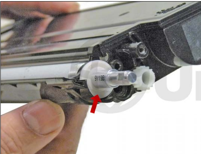
11. Remove the round bearings from both sides of the mag roller.
